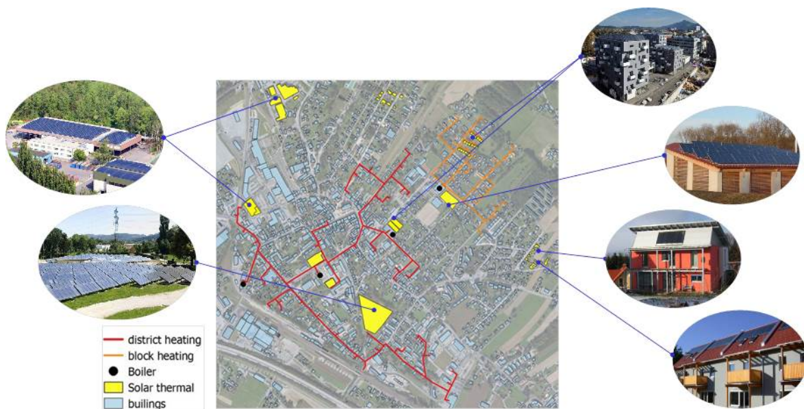
Figure 13: Overview over solar thermal system concepts in urban environments by means of a virtual study area
