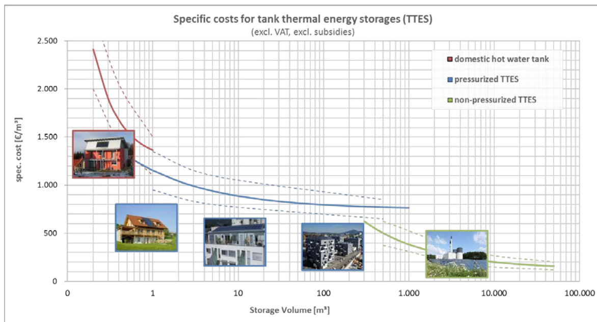
Figure 7: Cost curves for different tank thermal energy storage technologies (incl. insulation; excl. VAT, excl. subsidies)
