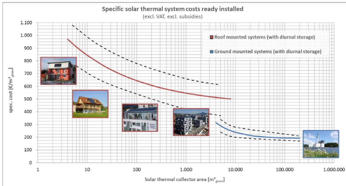
Figure 10: Cost curves for (ready installed) roof mounted and ground mounted solar thermal systems with diurnal storage (excl. VAT, excl. subsidies); red : roof-mounted ST systems with diurnal storage; blue : ground-mounted ST systems with diurnal storage
