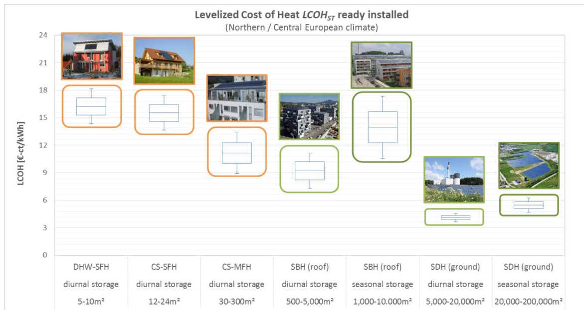
Figure 11: Typical range of LCOE_{ST} for ST generated heat per system category (reference: Central European climate)
