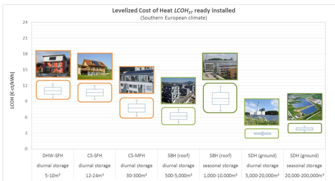
Figure 12: Typical range of LCOE_{ST} for ST generated heat per system category (reference: Southern European climate)
