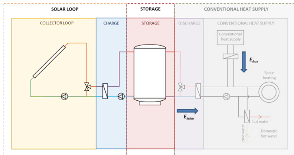
Figure 1: System boundaries for the solar thermal systems investigated
