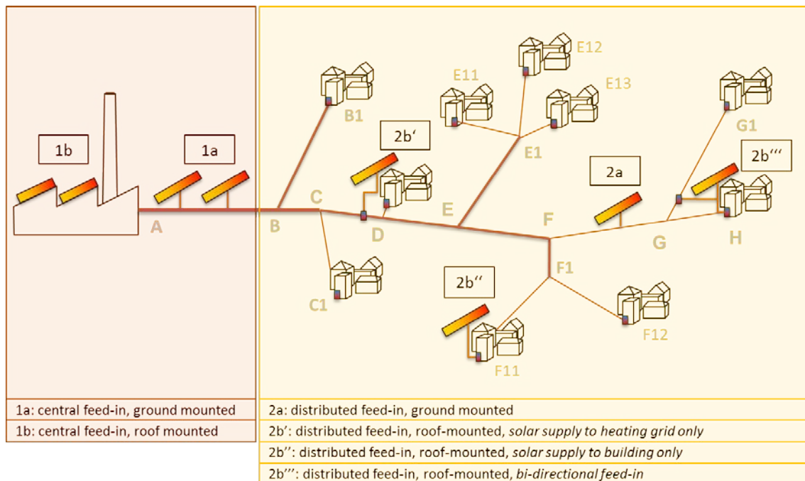
Figure 3: Integration options for solar thermal systems in district heating grids (source: AEE INTEC adapted from /12/)
