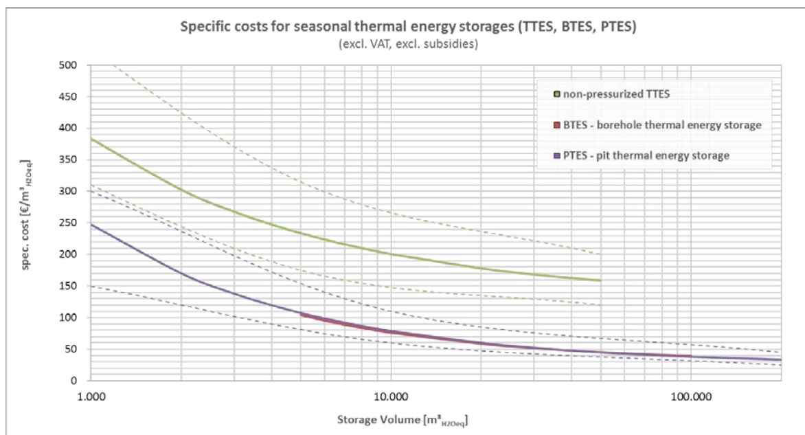
Figure 8: Cost curves for different long-term (seasonal) storage technologies (excl. VAT, excl. subsidies)
