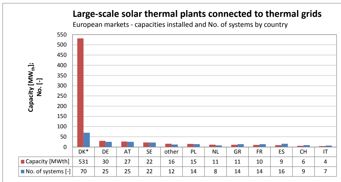
Figure 2: Large-scale solar thermal plants connected to thermal grids in Europe – capacities installed and No. of systems by end of 2014 (*Denmark: October 2015) (Data source: Dalenbäck J.-O. - Chalmers University of Technology, SE and Trier D. – PlanEnergi, DK)
