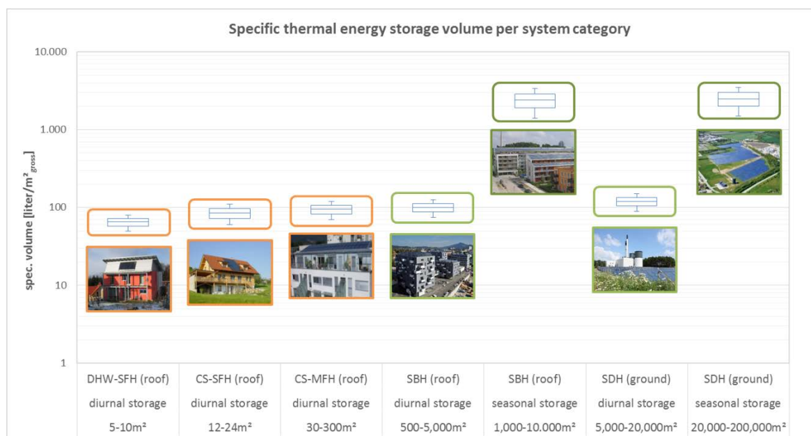
Figure 6: Specific thermal energy storage volume per solar thermal system category
