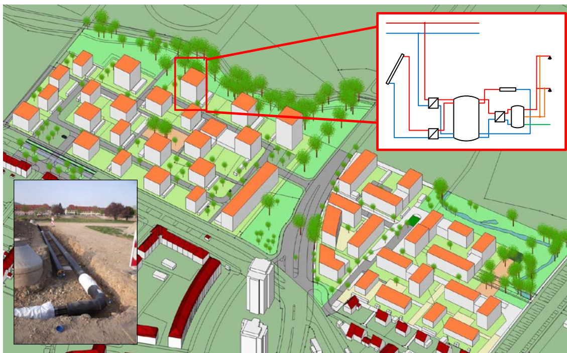
Figure 4: Schematic overview over the solar assisted block heating system in Freiburg- Glutleutmatten, DE (source: Fraunhofer ISE) (Details – based on design data: Total heated floor area: 40.000 m 2 / Total roof-mounted solar thermal system area: 2000 m 2 / Total solar energy storage volume: 160 m 3 / Total annual thermal energy demand: 2.200 MWh / Total annual solar energy yield: 660 MWh / Solar fraction: 20%)
