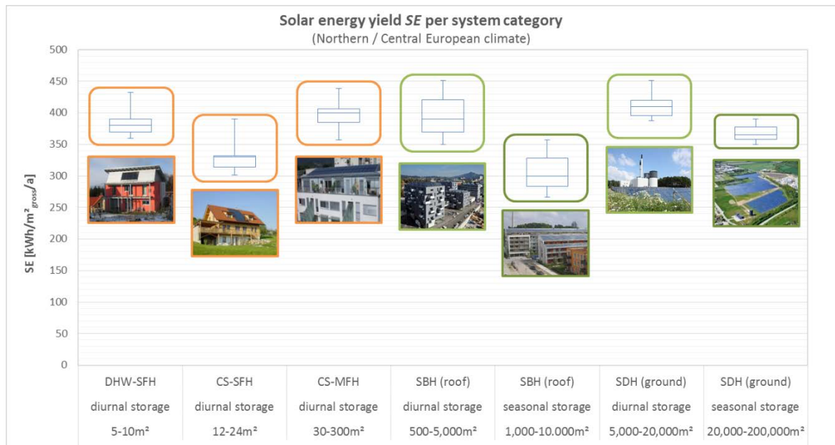
Figure 5: Solar energy yield per system category (valid for Central European climate)
