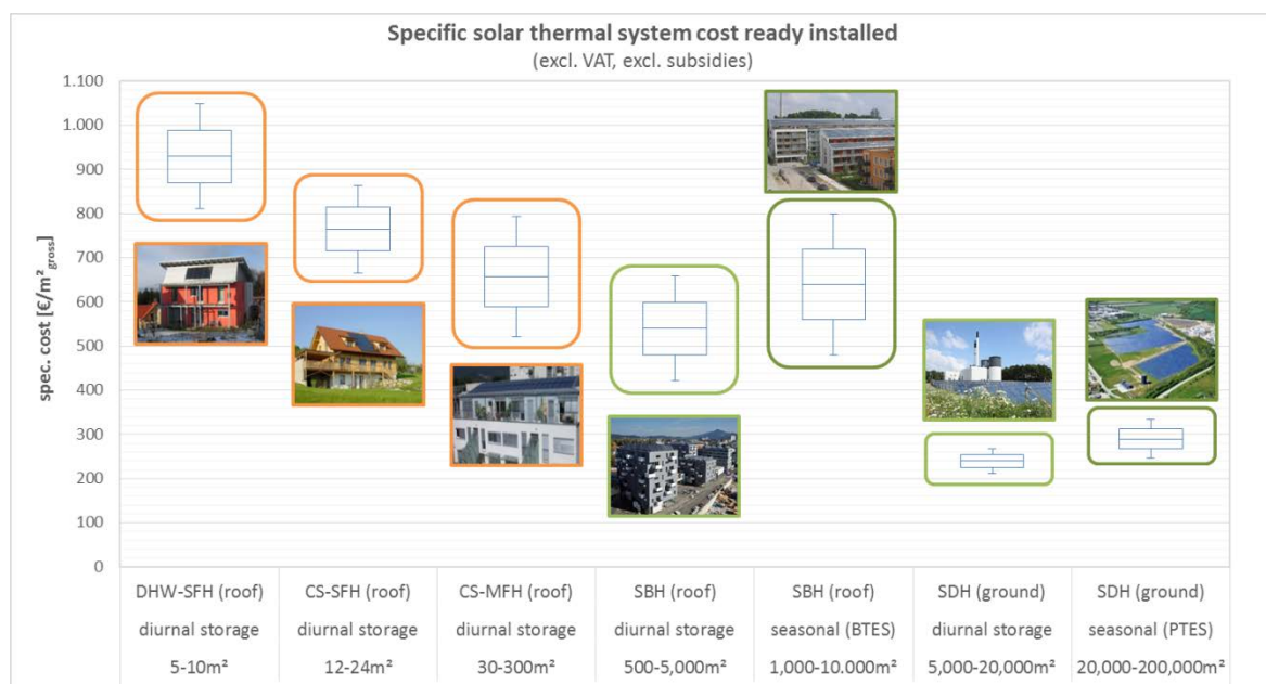
Figure 9: Typical range of specific costs per solar thermal system category ready installed (excl. VAT, excl. subsidies); orange: ST systems in single and multi-family homes with diurnal storage; light green: ST systems connected to thermal grids with diurnal storage; dark green: ST systems connected to thermal grids with seasonal storage
